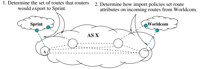
Figure 6. How rcc computes route propagation.
